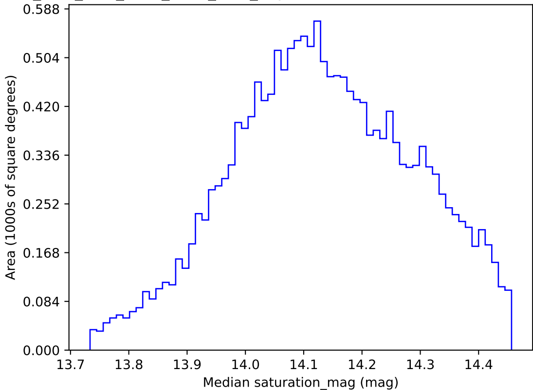
ddf_acor_sf15_lsf20_lsr20_v3.4_10yrs WFD z band: Median saturation_mag
