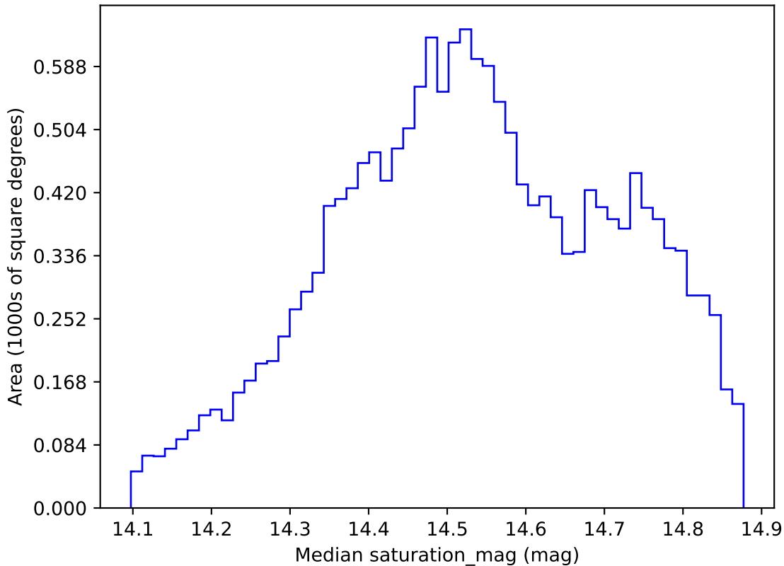
ddf_acor_sf15_lsf20_lsr20_v3.4_10yrs WFD i band: Median saturation_mag
