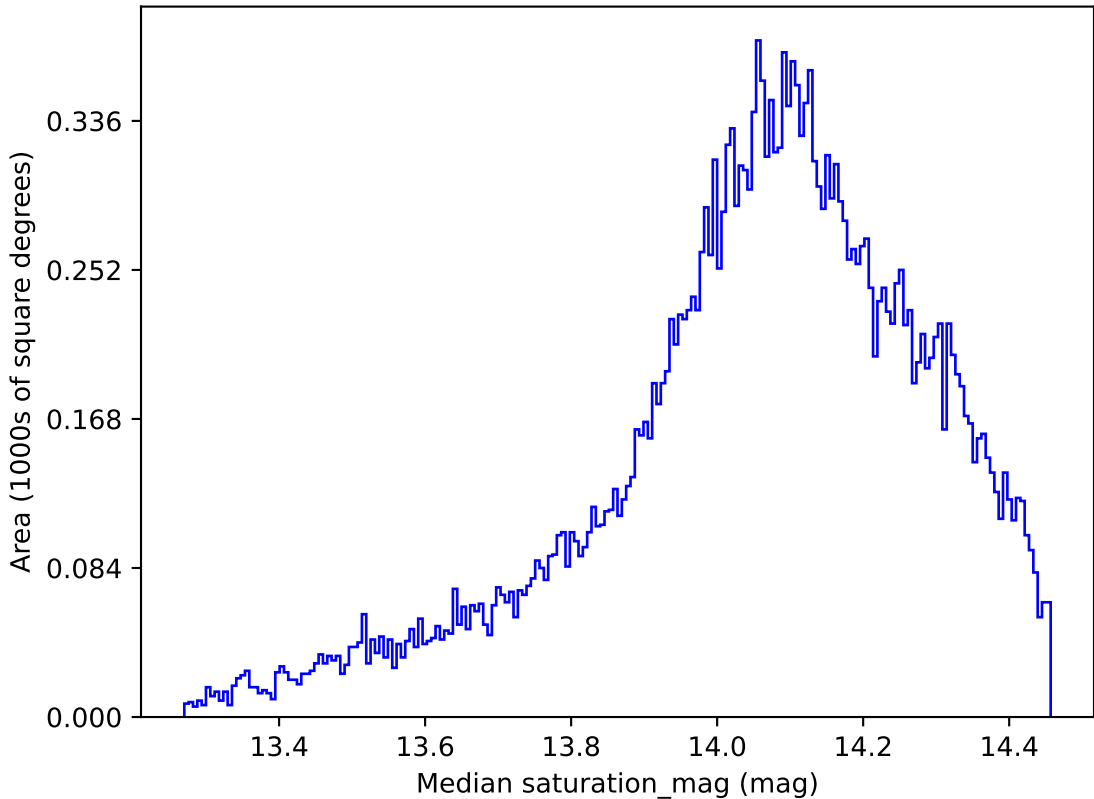
ddf_acor_sf15_lsf20_lsr20_v3.4_10yrs All sky z band: Median saturation_mag
