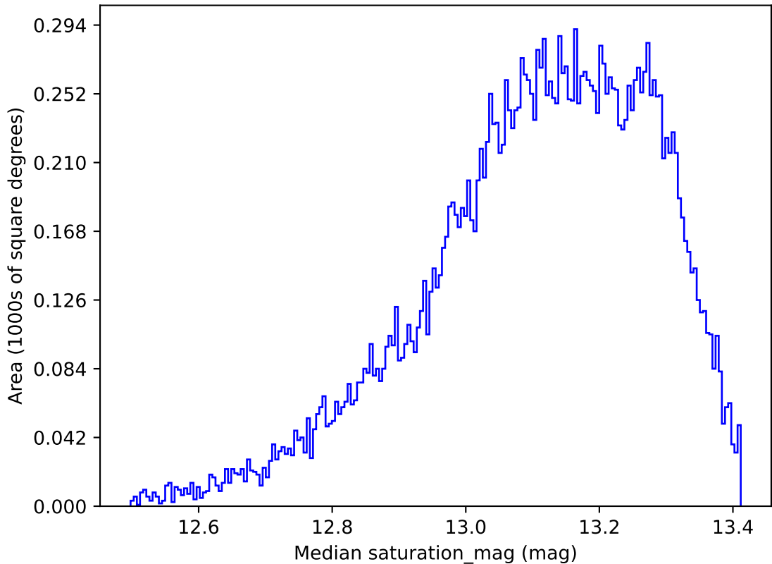
ddf_acor_sf15_lsf20_lsr20_v3.4_10yrs All sky y band: Median saturation_mag
