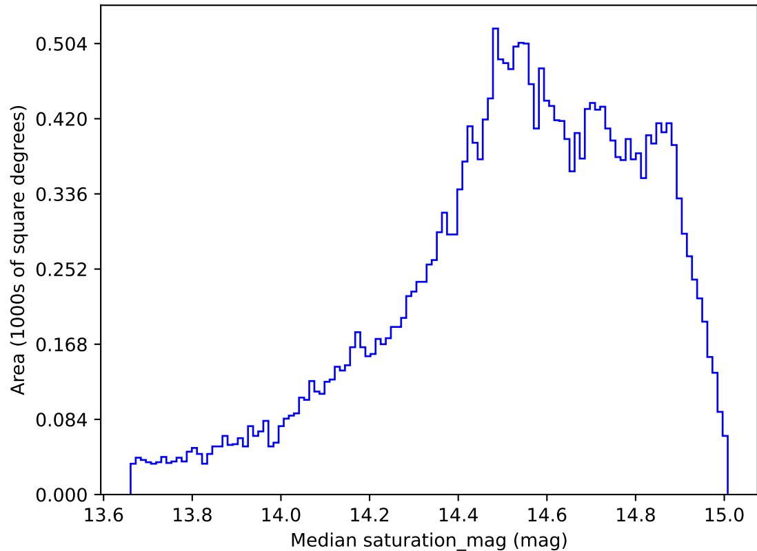
ddf_acor_sf15_lsf20_lsr20_v3.4_10yrs All sky r band: Median saturation_mag
