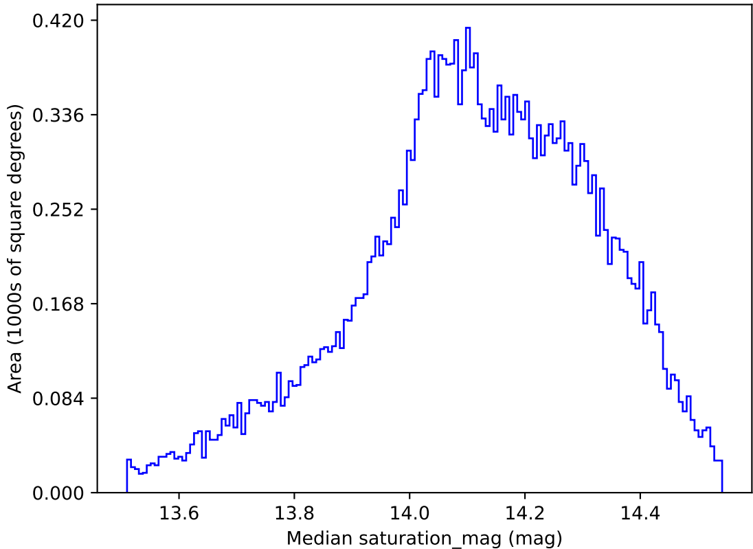
ddf_acor_sf15_lsf20_lsr20_v3.4_10yrs All sky all bands: Median saturation_mag
