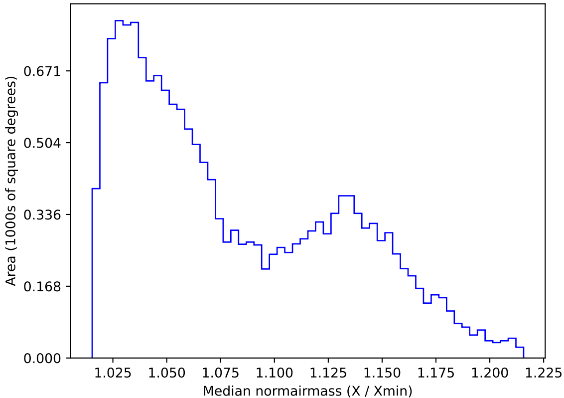
ddf_acor_sf15_lsf20_lsr20_v3.4_10yrs WFD g band: Median normairmass
