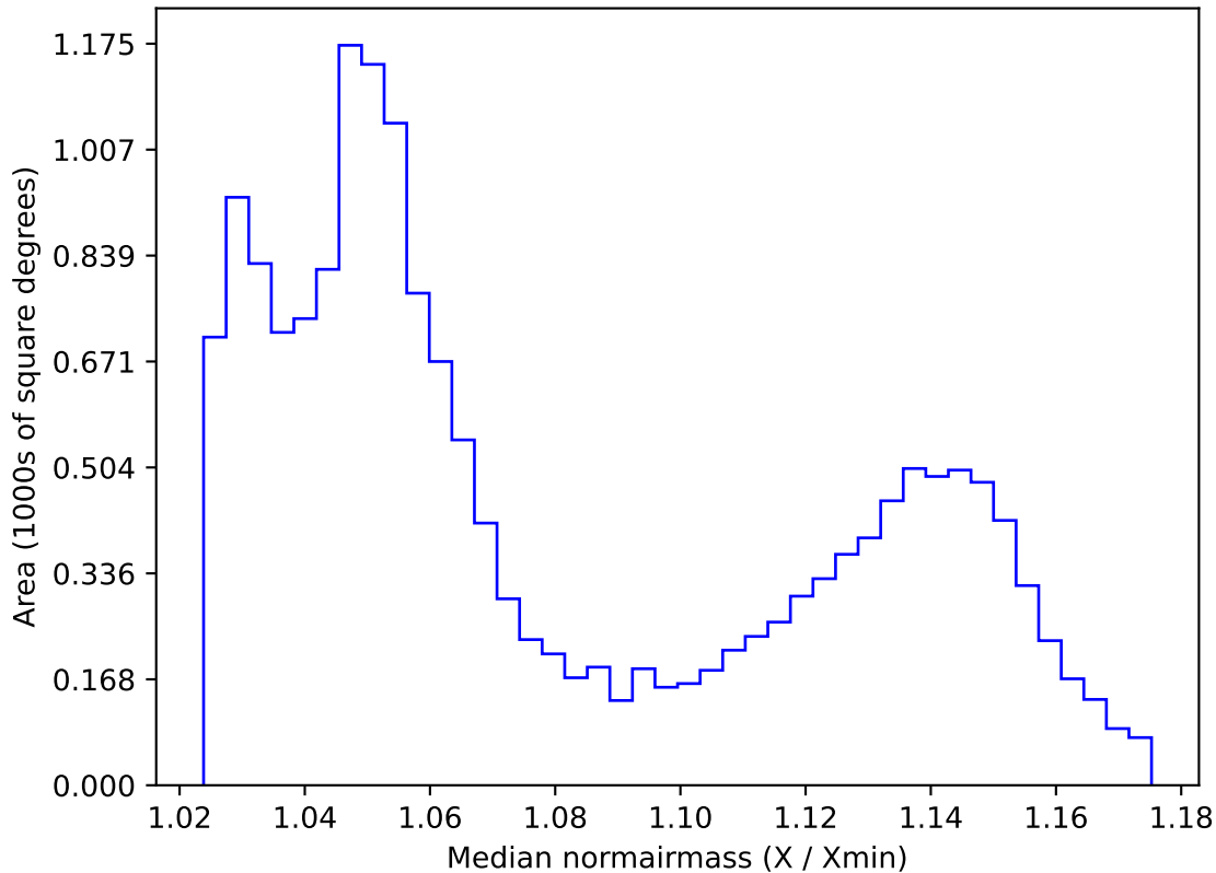
ddf_acor_sf15_lsf20_lsr20_v3.4_10yrs WFD all bands: Median normairmass
