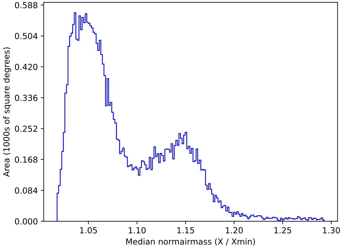
ddf_acor_sf15_lsf20_lsr20_v3.4_10yrs All sky z band: Median normairmass
