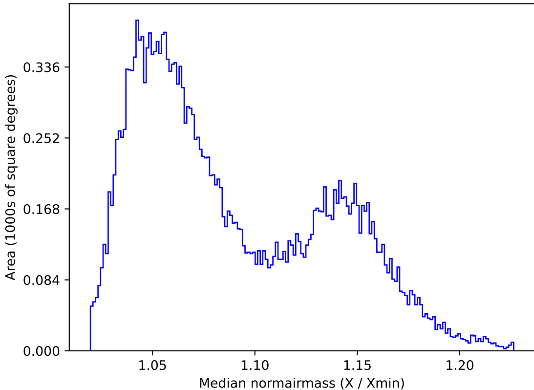
ddf_acor_sf15_lsf20_lsr20_v3.4_10yrs All sky y band: Median normairmass
