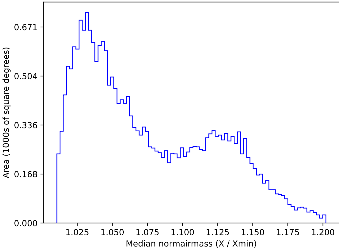
ddf_acor_sf15_lsf20_lsr20_v3.4_10yrs All sky u band: Median normairmass
