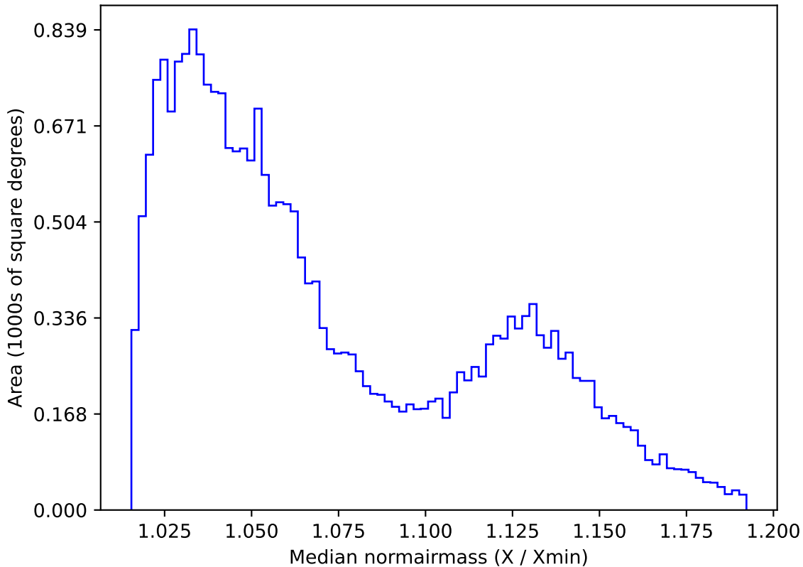
ddf_acor_sf15_lsf20_lsr20_v3.4_10yrs All sky r band: Median normairmass
