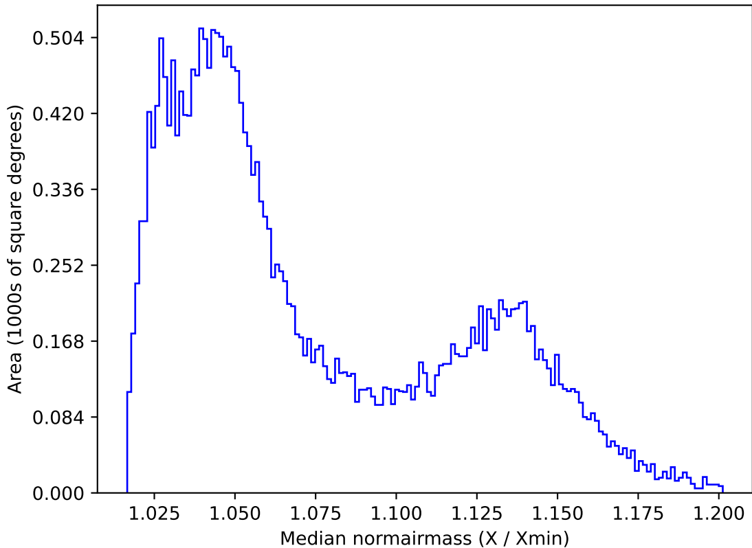
ddf_acor_sf15_lsf20_lsr20_v3.4_10yrs All sky i band: Median normairmass
