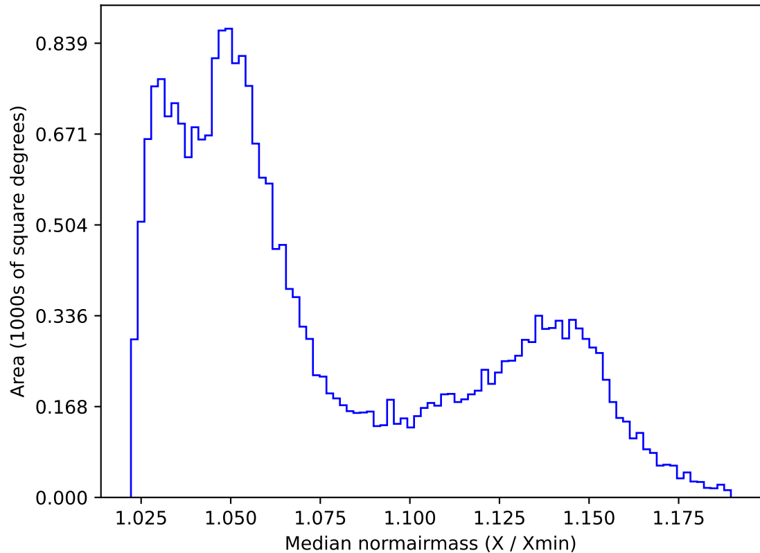
ddf_acor_sf15_lsf20_lsr20_v3.4_10yrs All sky all bands: Median normairmass
