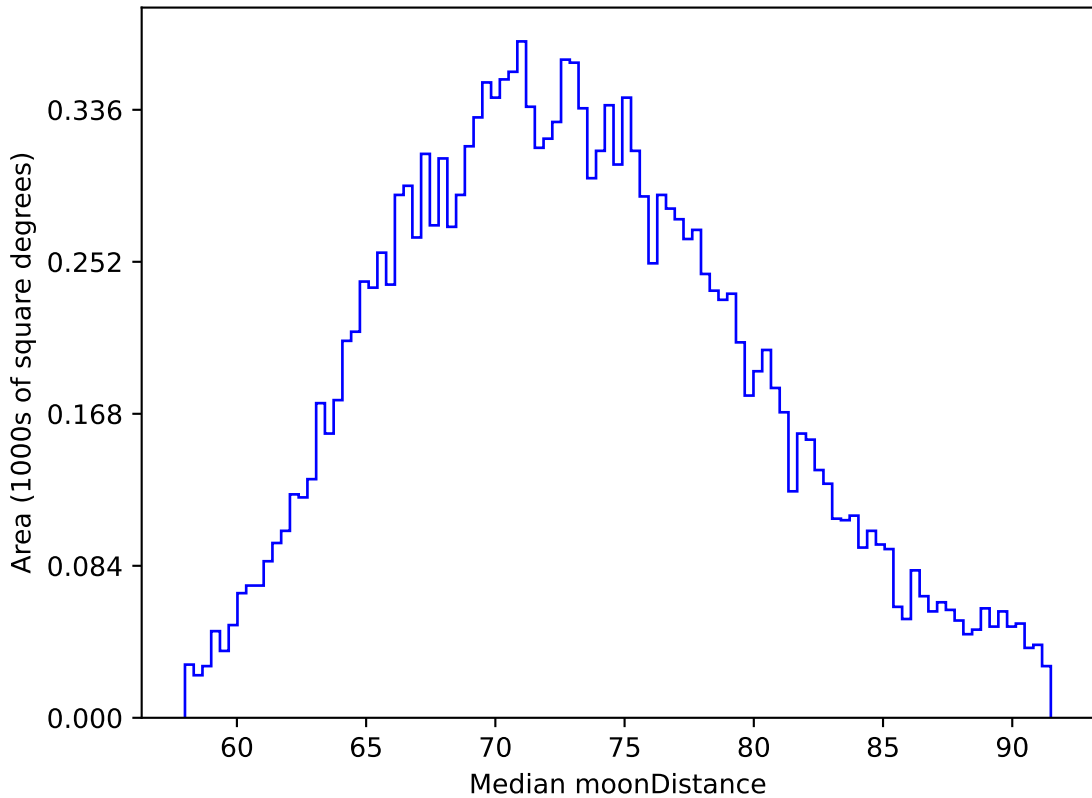
ddf_acor_sf15_lsf20_lsr20_v3.4_10yrs WFD z band: Median moonDistance
