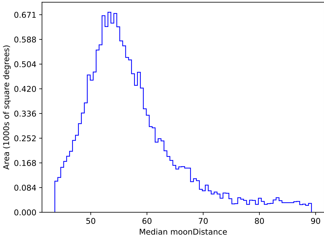
ddf_acor_sf15_lsf20_lsr20_v3.4_10yrs WFD y band: Median moonDistance
