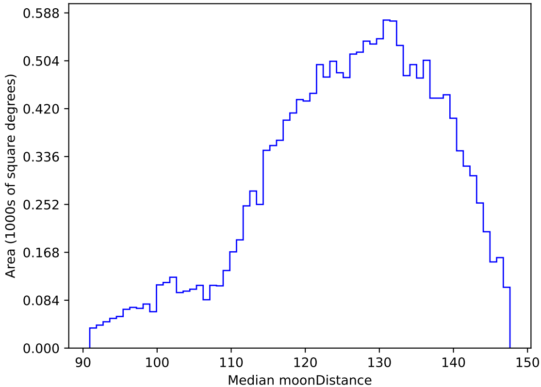
ddf_acor_sf15_lsf20_lsr20_v3.4_10yrs WFD u band: Median moonDistance
