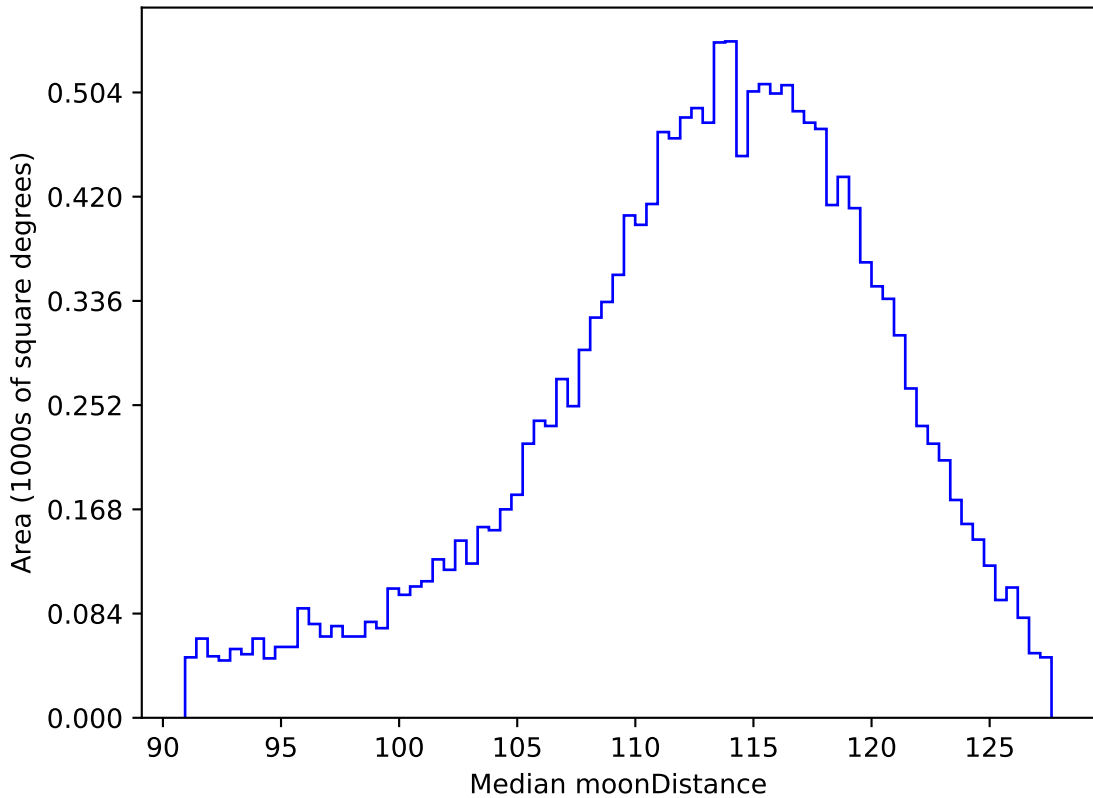
ddf_acor_sf15_lsf20_lsr20_v3.4_10yrs WFD r band: Median moonDistance
