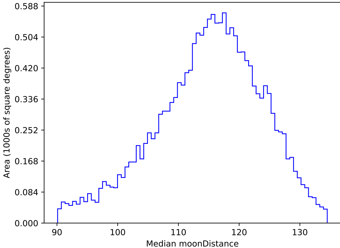
ddf_acor_sf15_lsf20_lsr20_v3.4_10yrs WFD g band: Median moonDistance
