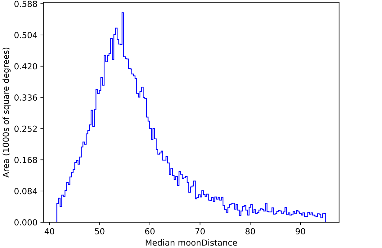
ddf_acor_sf15_lsf20_lsr20_v3.4_10yrs All sky y band: Median moonDistance
