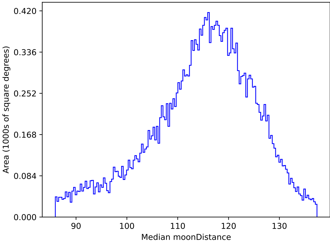
ddf_acor_sf15_lsf20_lsr20_v3.4_10yrs All sky g band: Median moonDistance
