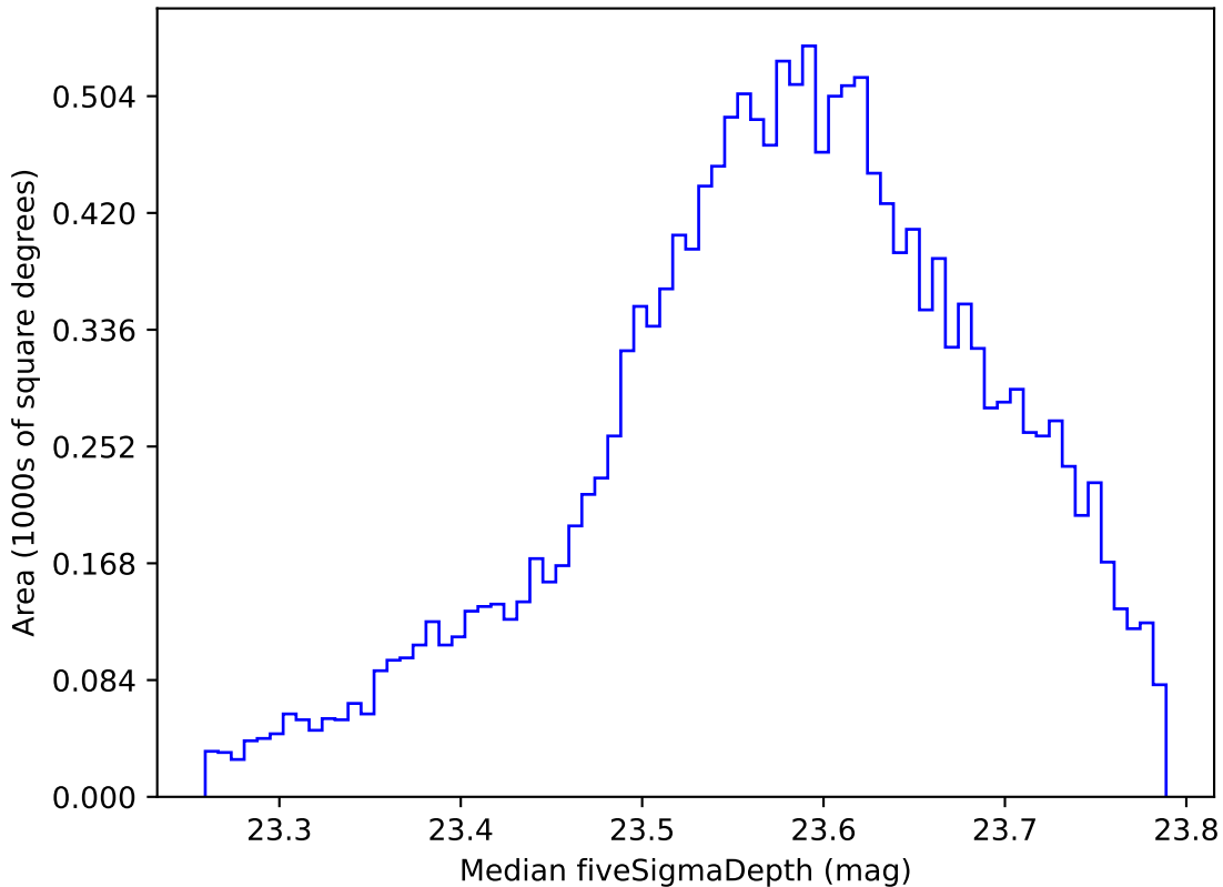
ddf_acor_sf15_lsf20_lsr20_v3.4_10yrs WFD i band: Median fiveSigmaDepth
