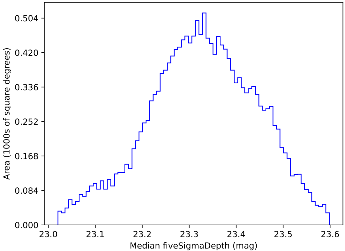
ddf_acor_sf15_lsf20_lsr20_v3.4_10yrs WFD all bands: Median fiveSigmaDepth
