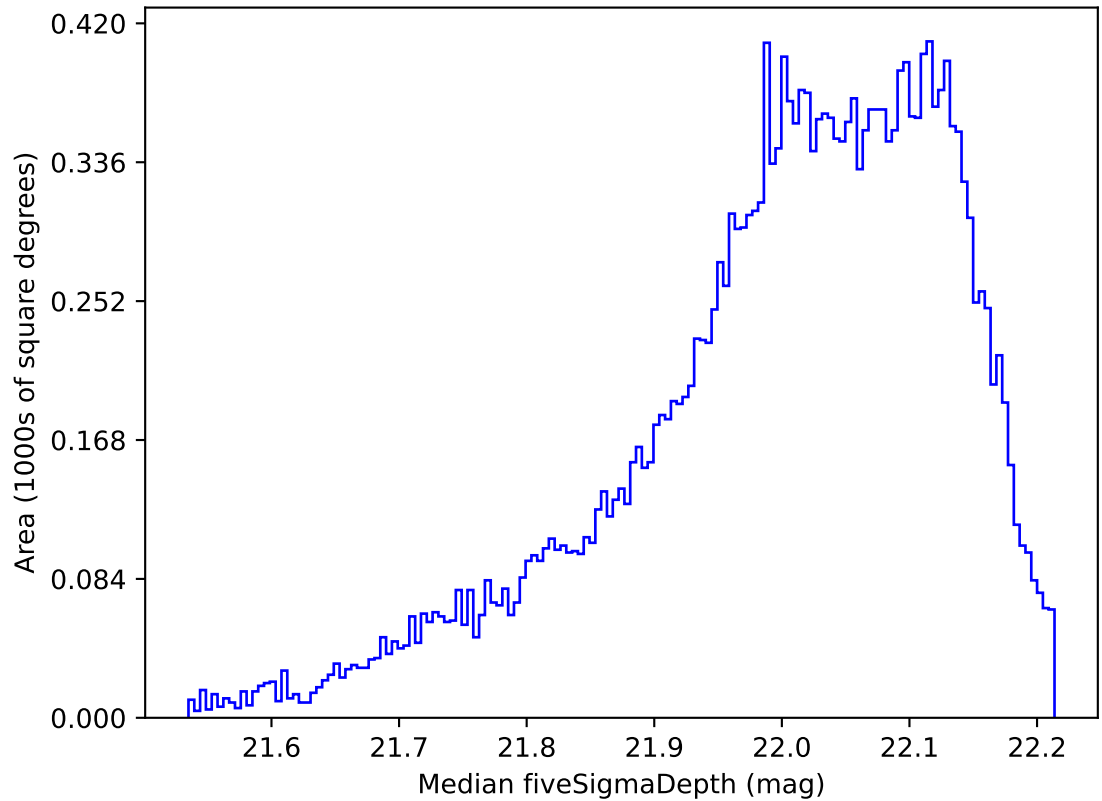
ddf_acor_sf15_lsf20_lsr20_v3.4_10yrs All sky y band: Median fiveSigmaDepth
