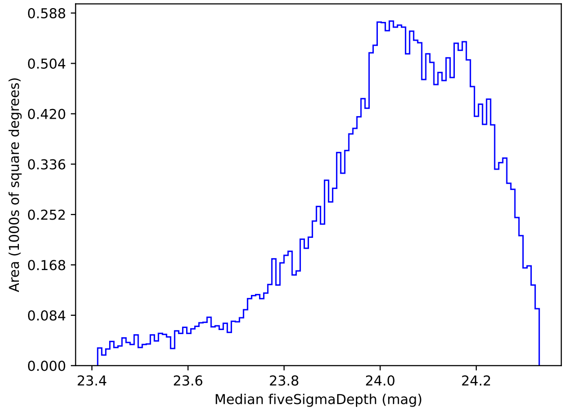
ddf_acor_sf15_lsf20_lsr20_v3.4_10yrs All sky r band: Median fiveSigmaDepth
