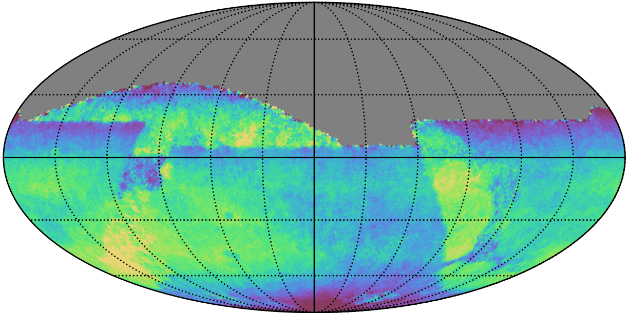
ddf_acor_sf15_lsf20_lsr20_v3.4_10yrs All sky all bands: Median fiveSigmaDepth
