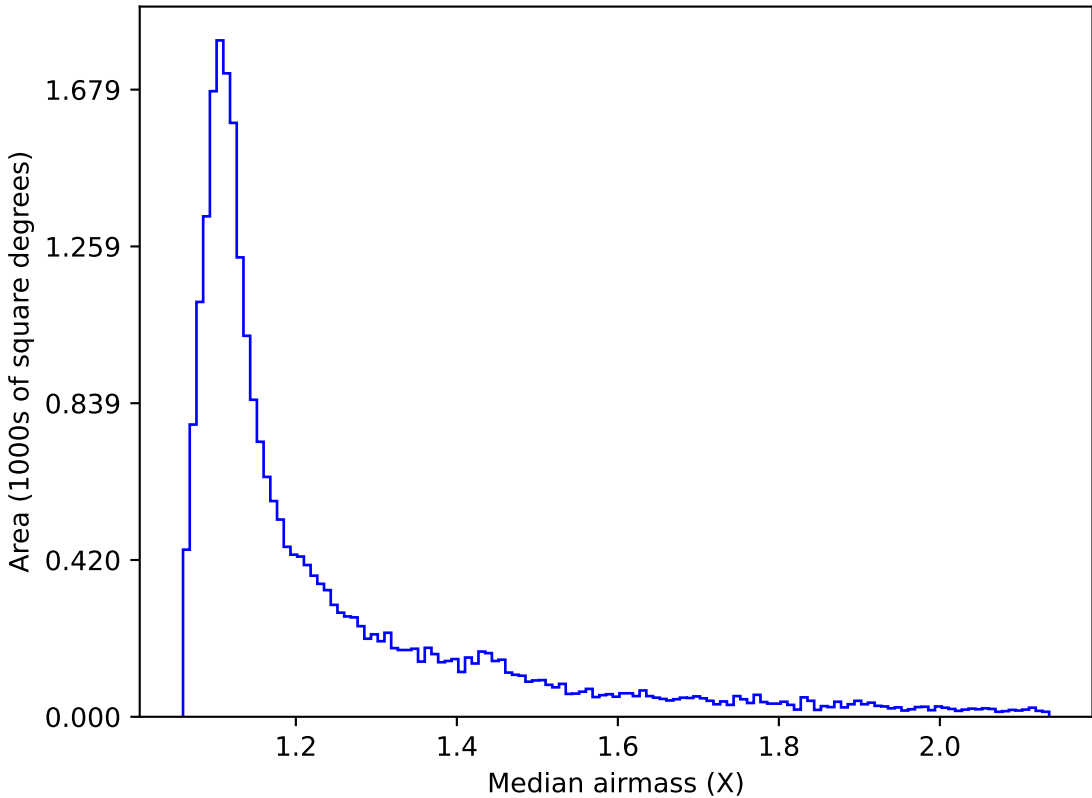
ddf_acor_sf15_lsf20_lsr20_v3.4_10yrs Yr 1 i band: Median airmass
