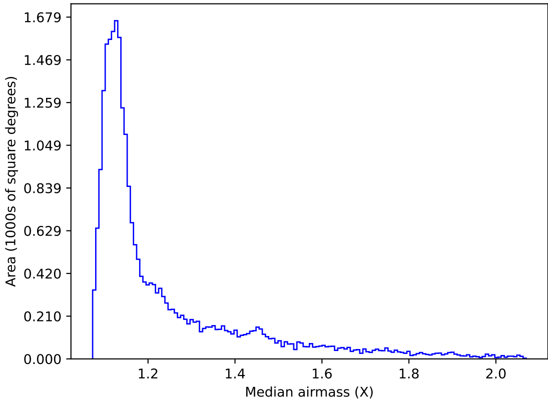
ddf_acor_sf15_lsf20_lsr20_v3.4_10yrs Yr 1 all bands: Median airmass
