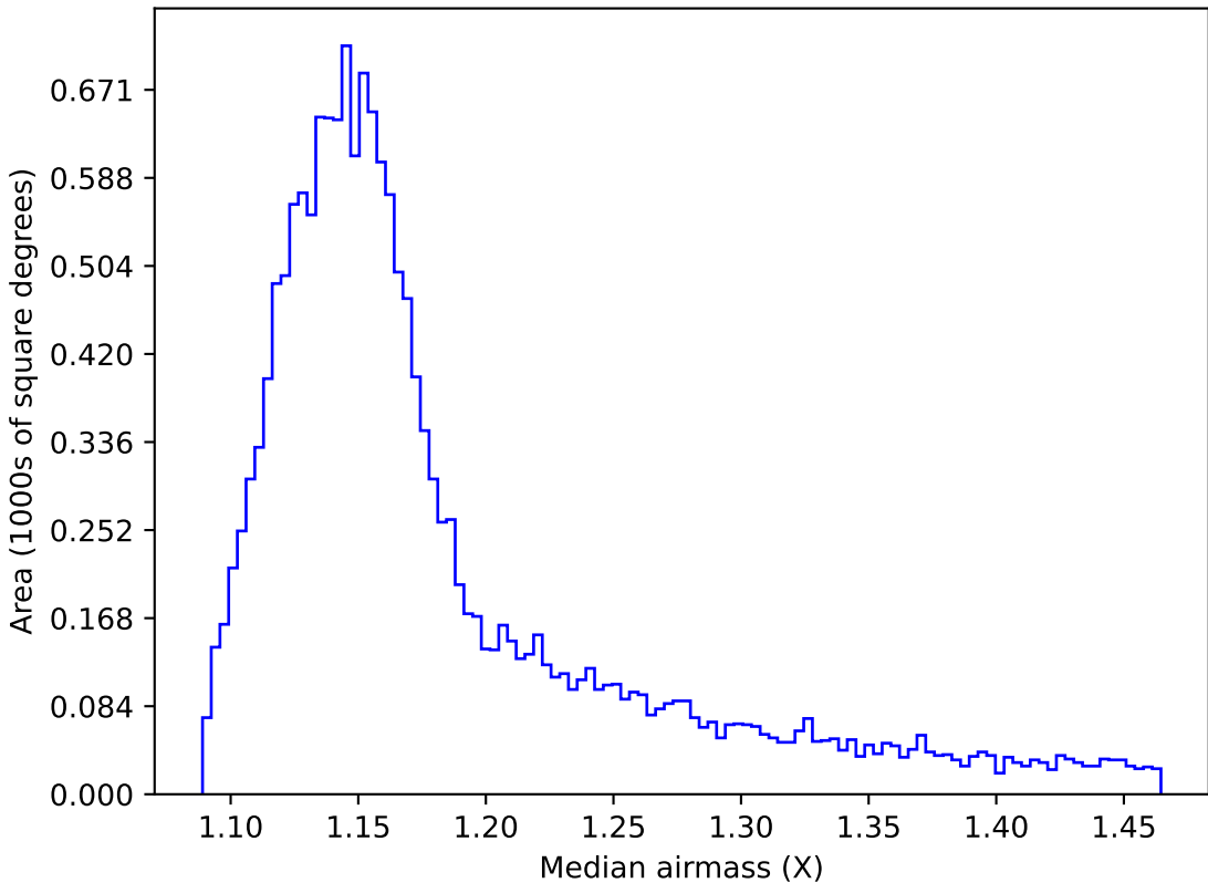
ddf_acor_sf15_lsf20_lsr20_v3.4_10yrs WFD z band: Median airmass
