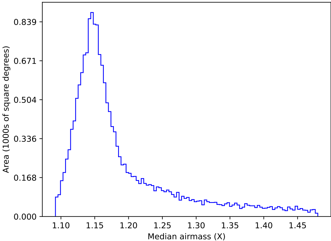
ddf_acor_sf15_lsf20_lsr20_v3.4_10yrs WFD y band: Median airmass
