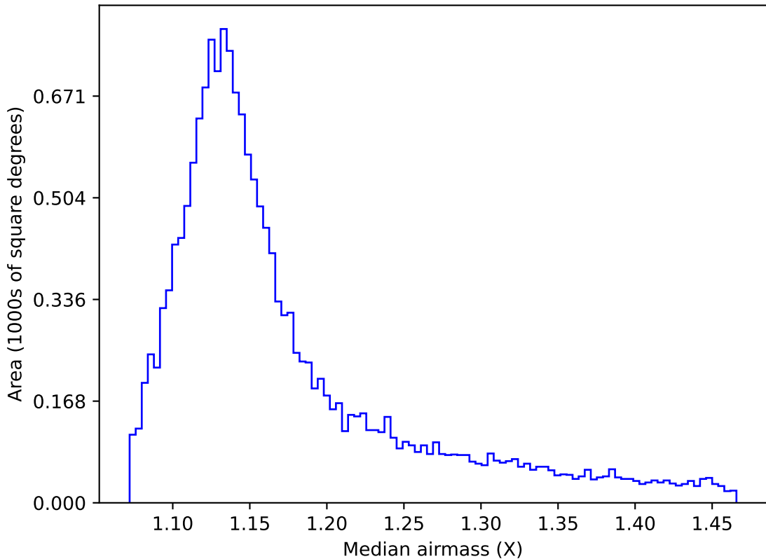
ddf_acor_sf15_lsf20_lsr20_v3.4_10yrs WFD u band: Median airmass
