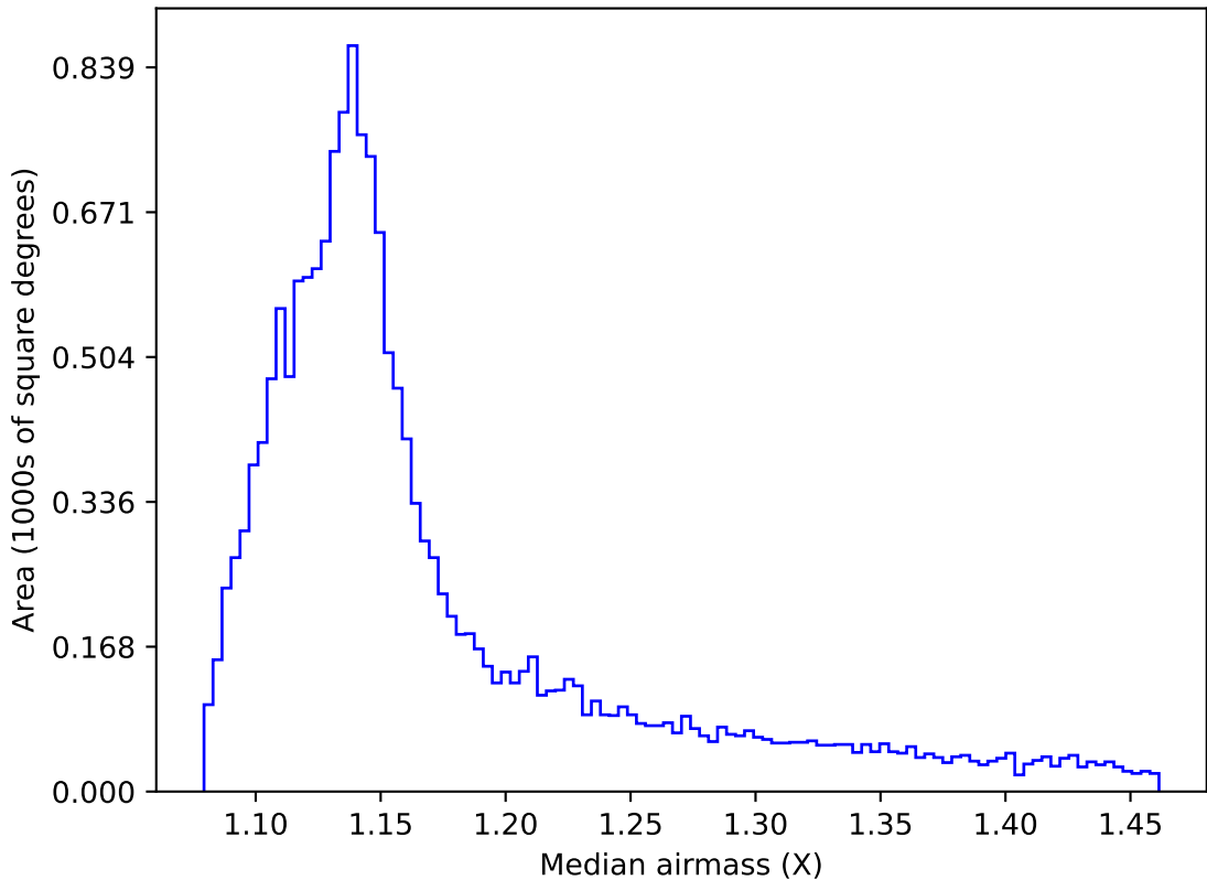
ddf_acor_sf15_lsf20_lsr20_v3.4_10yrs WFD i band: Median airmass
