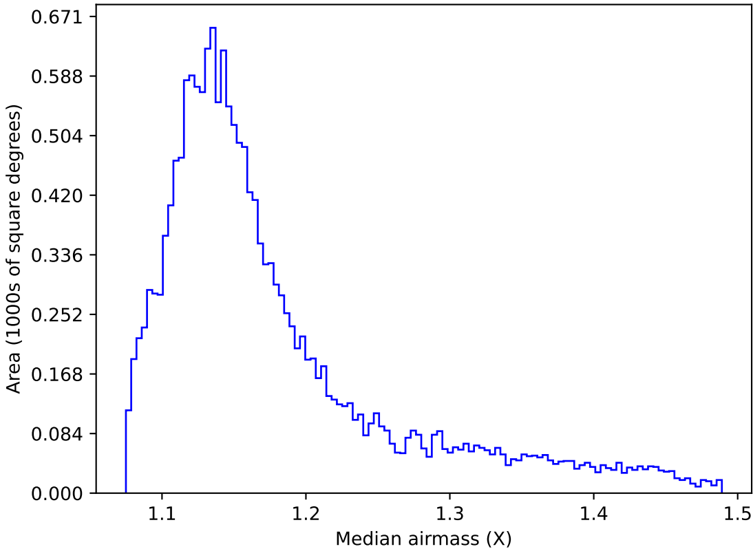
ddf_acor_sf15_lsf20_lsr20_v3.4_10yrs WFD g band: Median airmass
