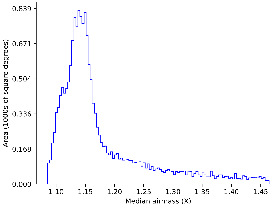
ddf_acor_sf15_lsf20_lsr20_v3.4_10yrs WFD all bands: Median airmass
