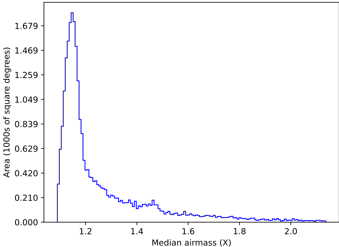
ddf_acor_sf15_lsf20_lsr20_v3.4_10yrs All sky z band: Median airmass
