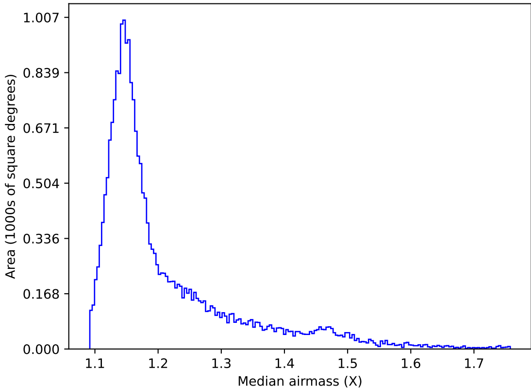
ddf_acor_sf15_lsf20_lsr20_v3.4_10yrs All sky y band: Median airmass
