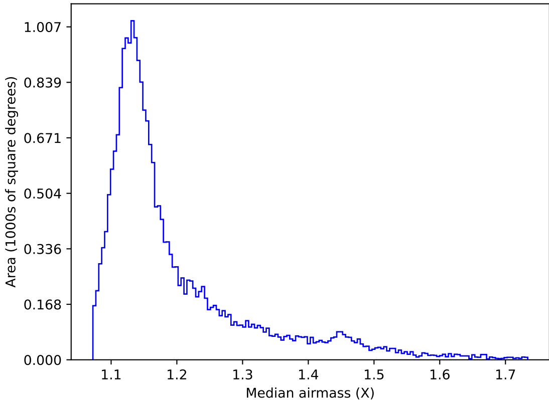
ddf_acor_sf15_lsf20_lsr20_v3.4_10yrs All sky u band: Median airmass
