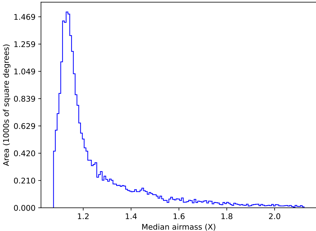
ddf_acor_sf15_lsf20_lsr20_v3.4_10yrs All sky g band: Median airmass
