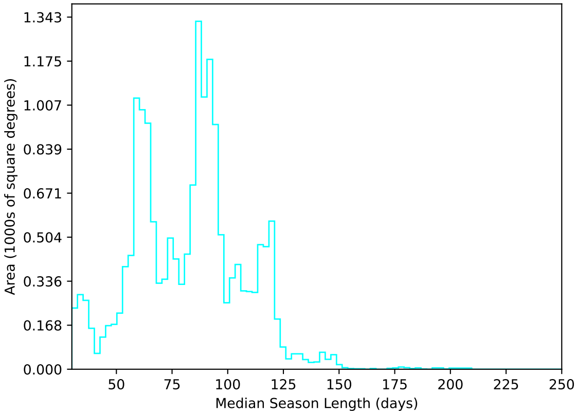
ddf_acor_sf15_ls20_lsr20_v3.4_10yrs WFD u band: Median Season Length
