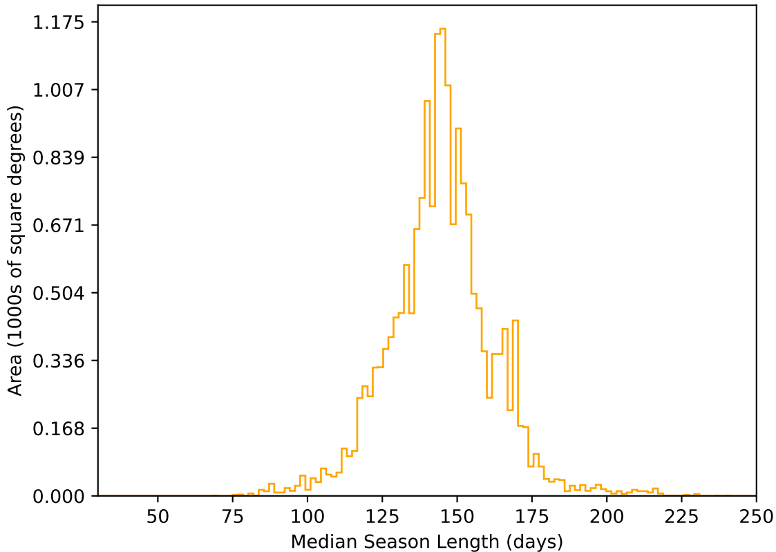
ddf_acor_sf15_lsf20_lsr20_v3.4_10yrs WFD r band: Median Season Length
