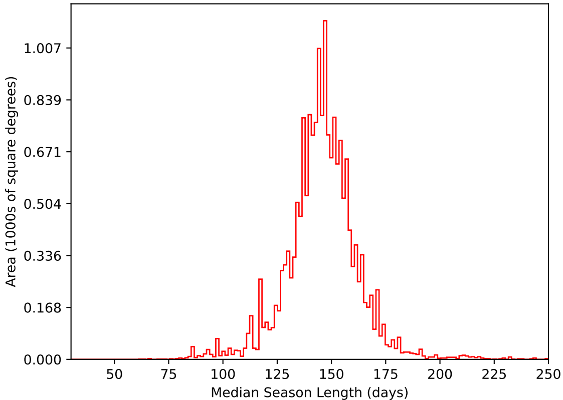
ddf_acor_sf15_lsf20_lsr20_v3.4_10yrs WFD i band: Median Season Length
