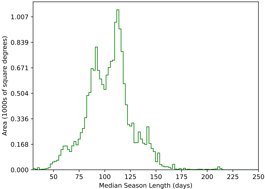
ddf_acor_sf15_lsf20_lsr20_v3.4_10yrs WFD g band: Median Season Length
