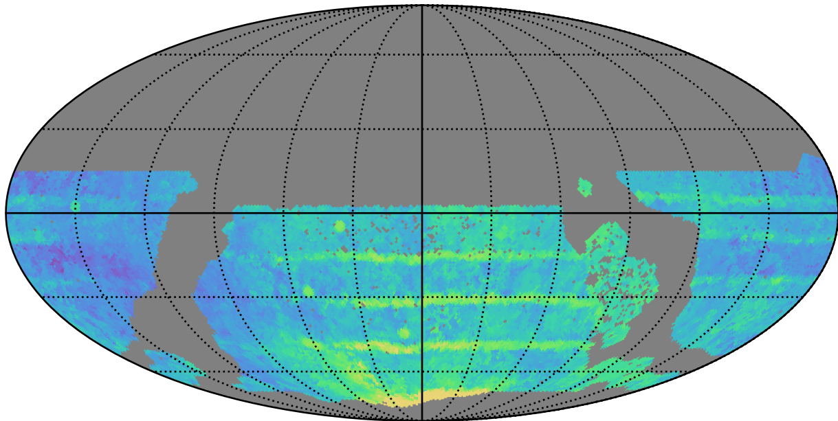
ddf_acor_sf15_lsf20_lsr20_v3.4_10yrs WFD all bands: Median Season Length
