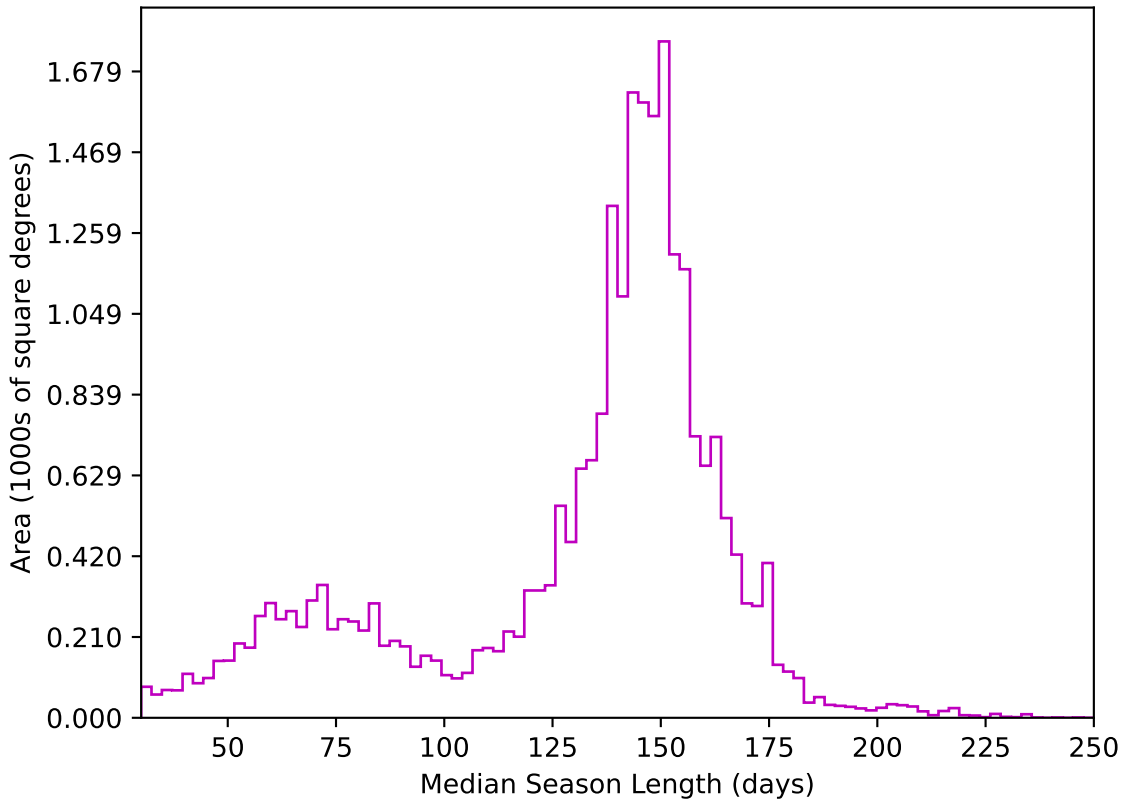
ddf_acor_sf15_lsf20_lsr20_v3.4_10yrs All sky z band: Median Season Length
