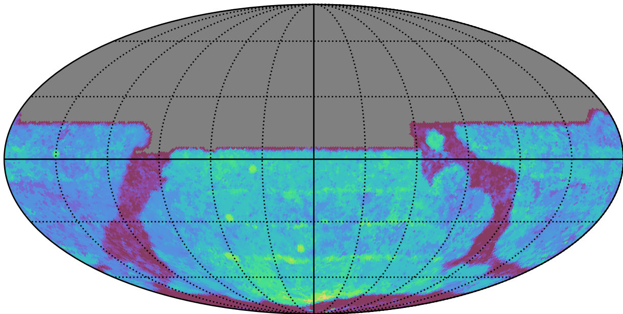
ddf_acor_sf15_lsf20_lsr20_v3.4_10yrs All sky y band: Median Season Length
