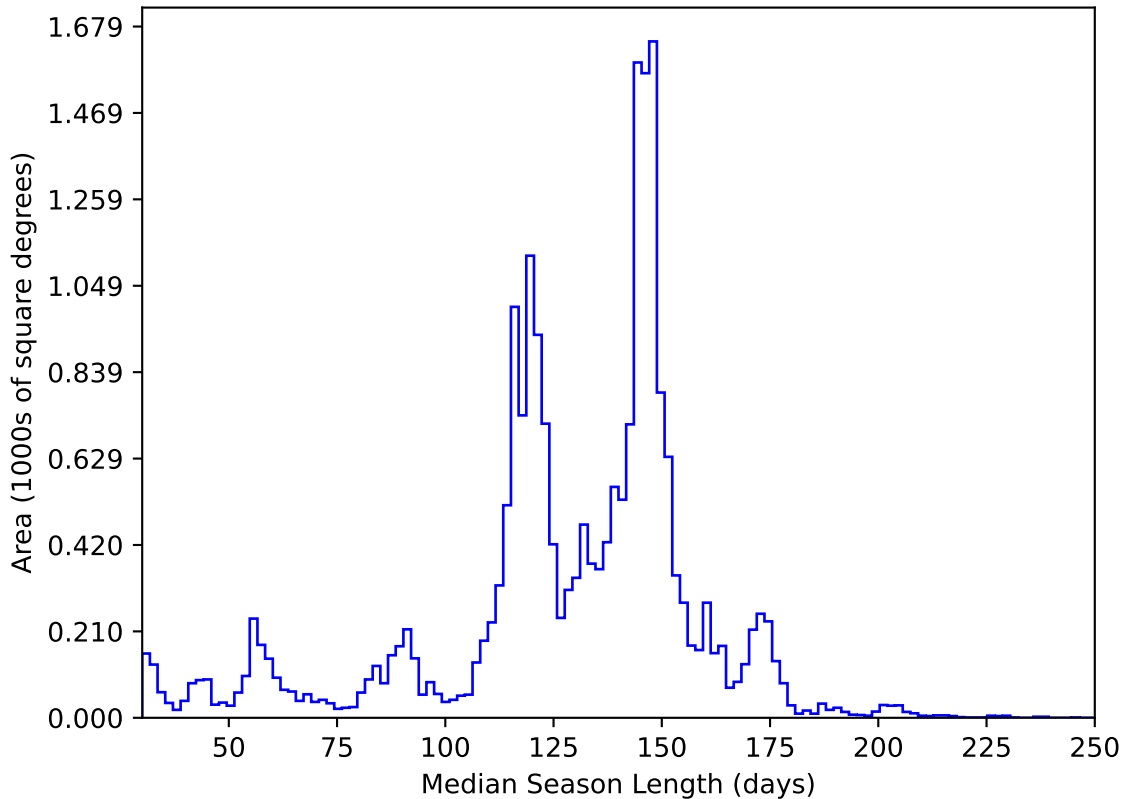
ddf_acor_sf15_lsf20_lsr20_v3.4_10yrs All sky y band: Median Season Length
