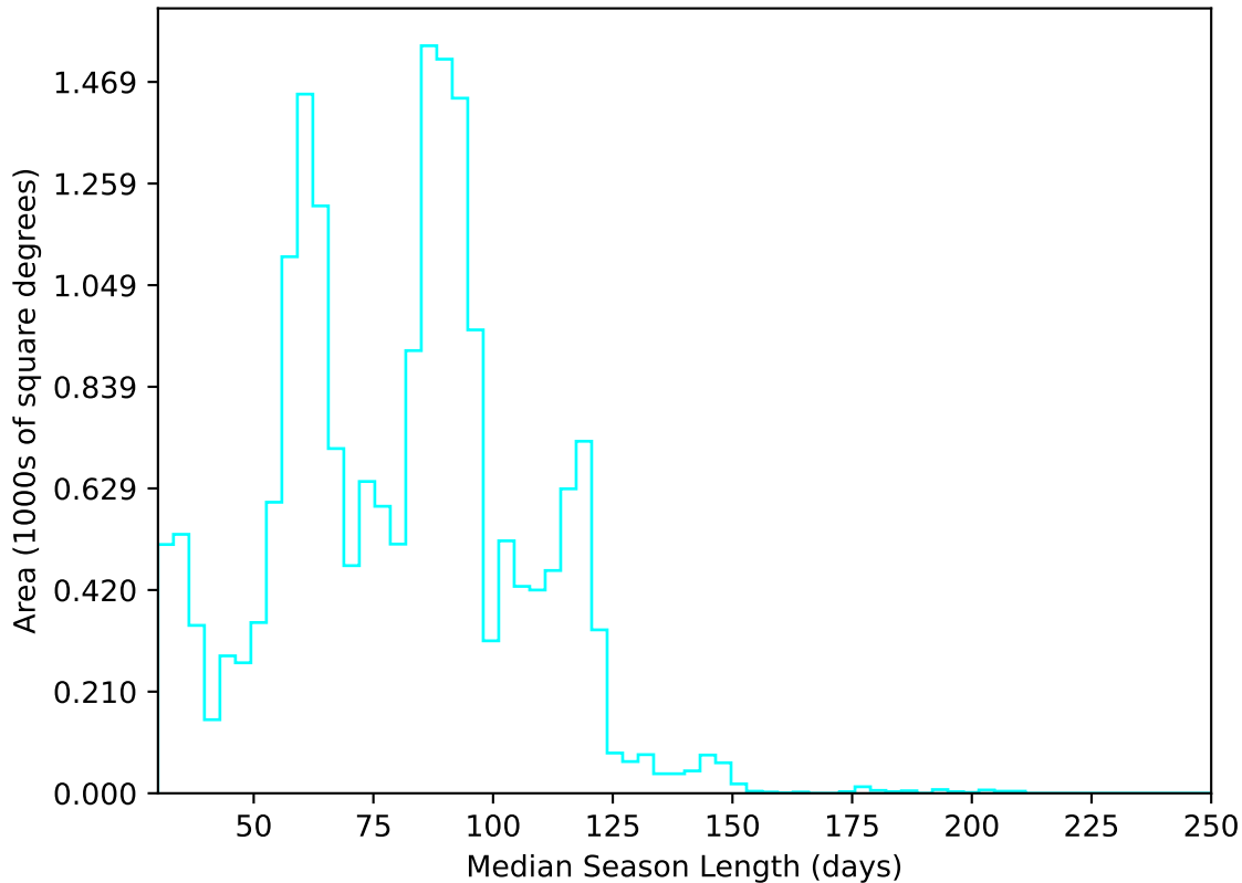
ddf_acor_sf15_lsf20_lsr20_v3.4_10yrs All sky u band: Median Season Length
