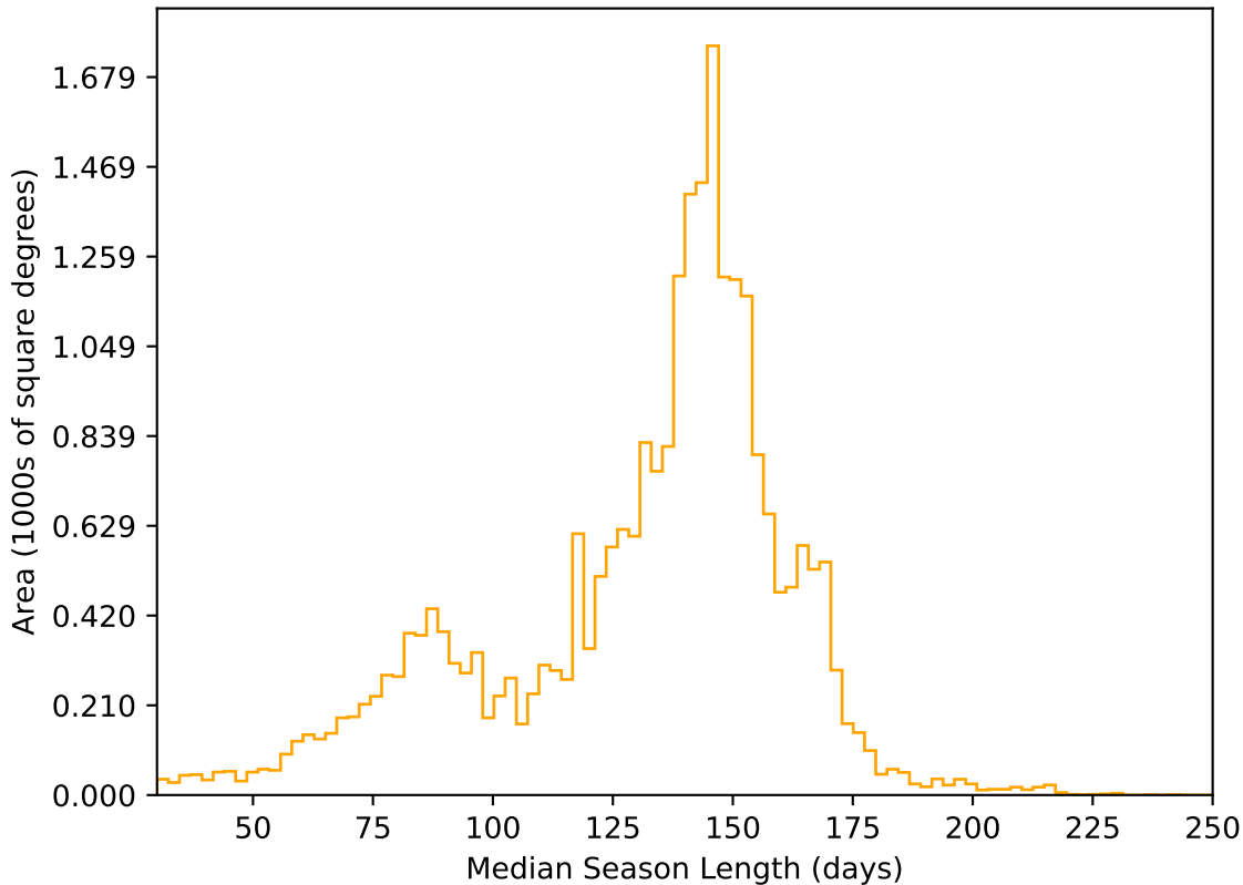
ddf_acor_sf15_lsf20_lsr20_v3.4_10yrs All sky r band: Median Season Length
