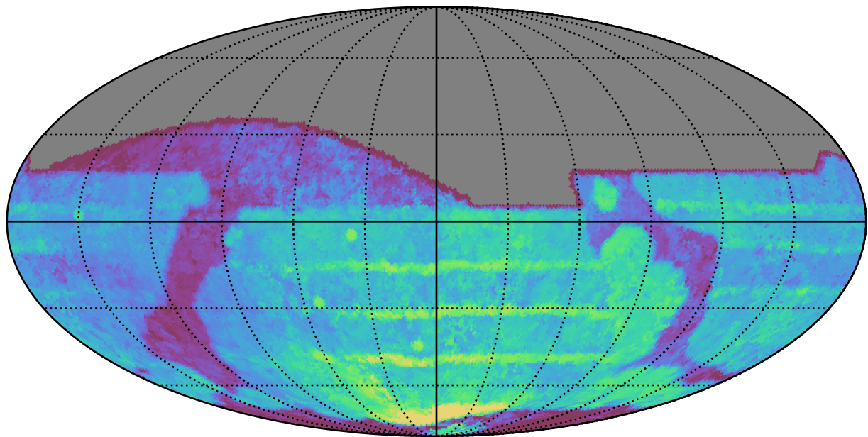
ddf_acor_sf15_lsf20_lsr20_v3.4_10yrs All sky all bands: Median Season Length
