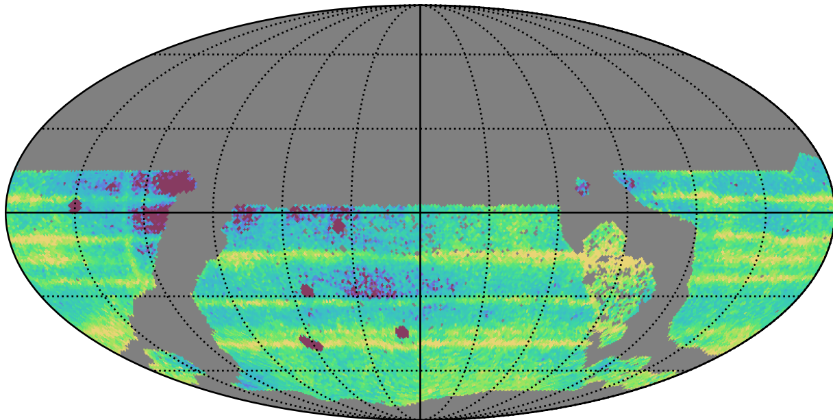
ddf_acor_sf15_lsf20_lsr20_v3.4_10yrs WFD: Median Intra-Night Gap
